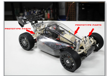
Additional prototype parts being functionally tested on Race Runner V4.
