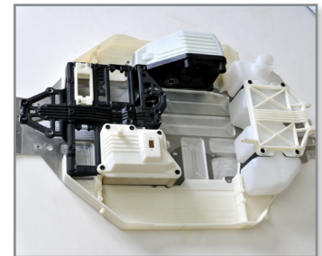
Assembly made up completely of prototypes except chassis and gas tank.
