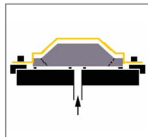
Figure 16: Blow release forces air between tool and formed part.
