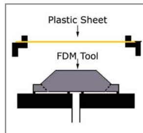
Figure 10: Thermoplastic sheet is clamped in frame.
