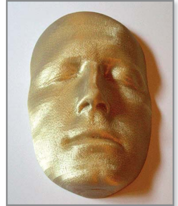
Figure 6: FDM tool, made in PPSF/PPSU, has formed more than 500 parts with no sign of wear
