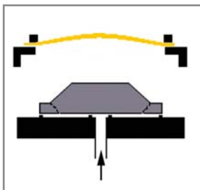
Figure 12: Air is forced upward for the material pre-stretch.
