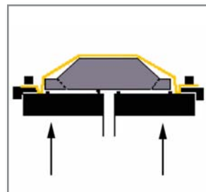
Figure 13: The tool rises, pressing into the sheet.
