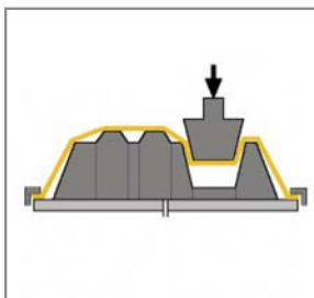
Figure 15: Plug pushes into sheet and tool cavity.
