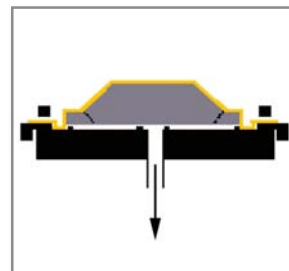
Figure 14: Vacuum is drawn to remove air from between the tool and sheet.
