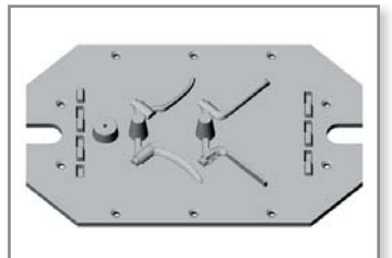
Figure 7: Matchplate (cope side shown) with mounting holes, alignment locators, gates, risers and sprue mounting pad.
