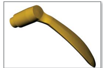
Figure 5: CAD file of door handle with draft and shrinkage allowance
